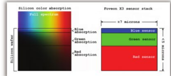
Foveon X3
